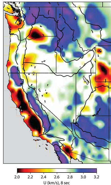
A map showing variation of Rayleigh wave (a type of seismic surface wave) group velocity for 8 sec period vibrations derived from more than 60,000 measurements. By cross correlating up to three years of continuous data from 512 western U.S. stations, including the EarthScope USArray Transportable Array and regional seismic networks, inter-station propagation velocities for all available station pairs were recovered and inverted for regional velocity structure. Thick black lines define major tectonic province boundaries. (Image courtesy of M.P. Moschetti, M.H. Ritzwoller, and N.M. Shapiro.)
